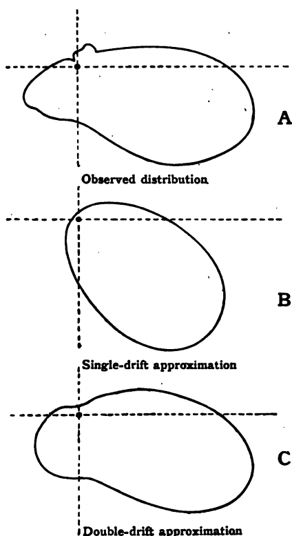
FIG. 8.—Observed and Calculated Distributions of Proper Motions. (Boss, Region VIII.)
